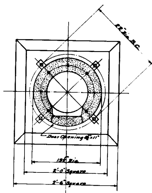
Plan of Base.
